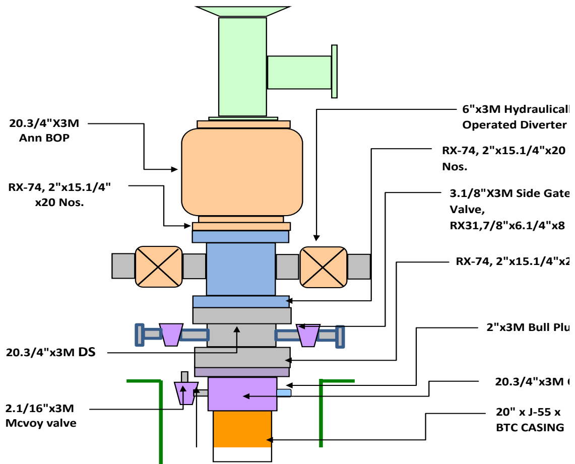
Figure No-3: Well Head & BOP Stack for Drilling 17.1/2" Hole
