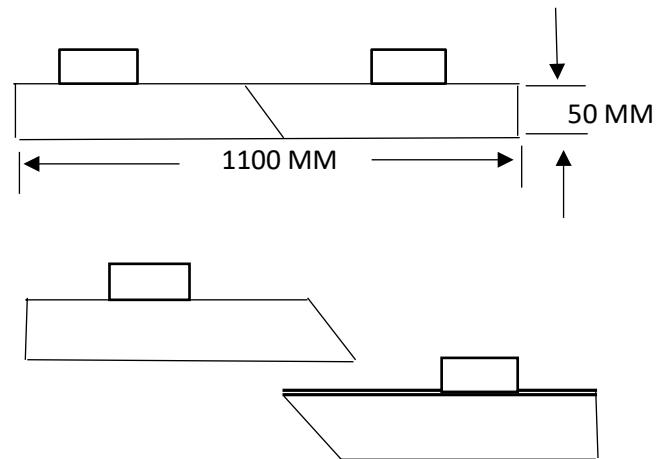
SIDE VIEW OF BOTTOM COVER & TOP COVER
