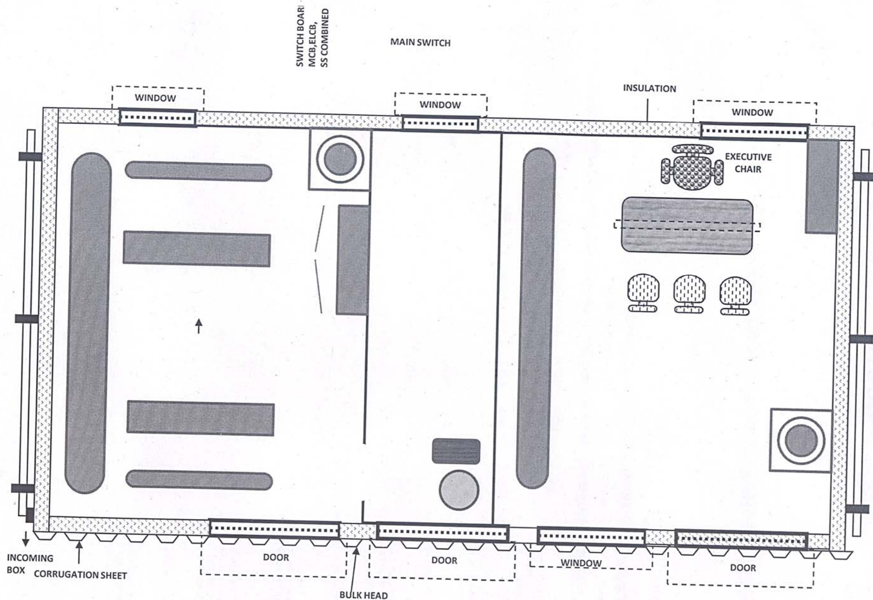
INTERNAL LAYOUT PLAN OF BUNK HOUSE
