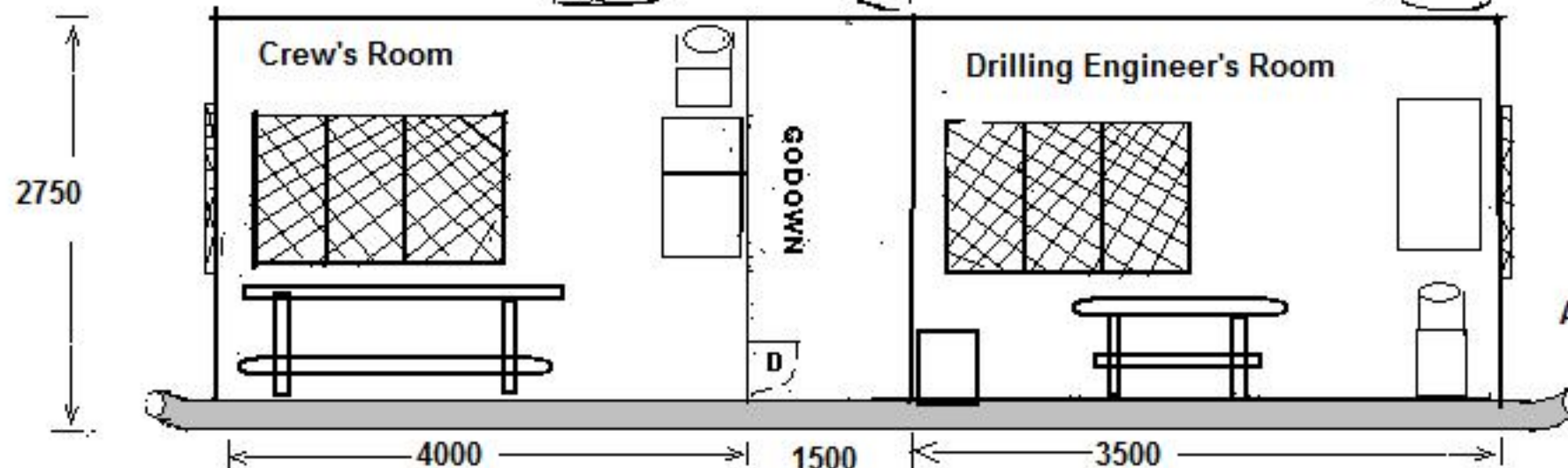
SECTIONAL VIEW
