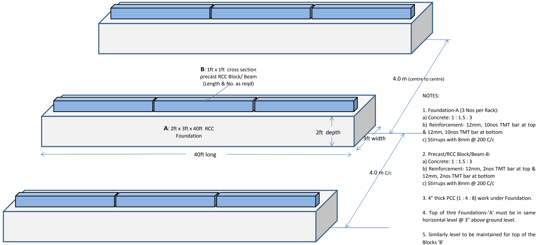
SCHEMATIC DRAWING OF FOUNDATION &amp; PRECAST/RCC BLOCK/BYAM FOR ONE CASING PIPE RACK
