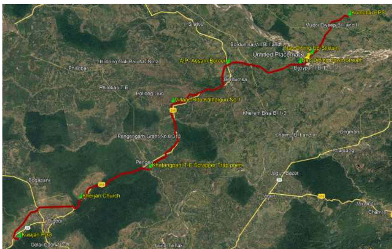
Fig: Showing entire pipeline route from Kumchai EPS to Kusijan FGS.
