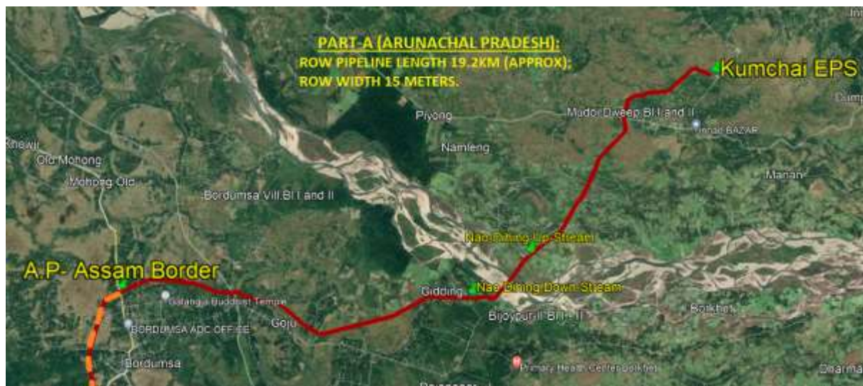
Fig: Showing only the Pipeline route of PART-A i.e from Kumchai EPS to A.P –Assam Border.
