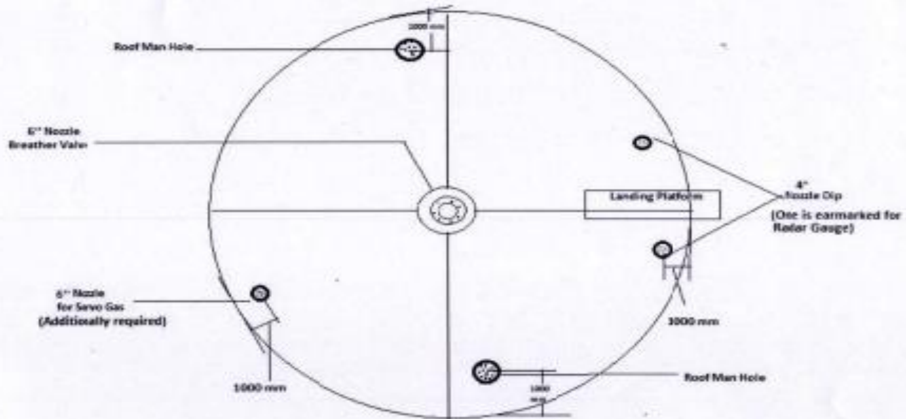
Fig(a): Tank top view
