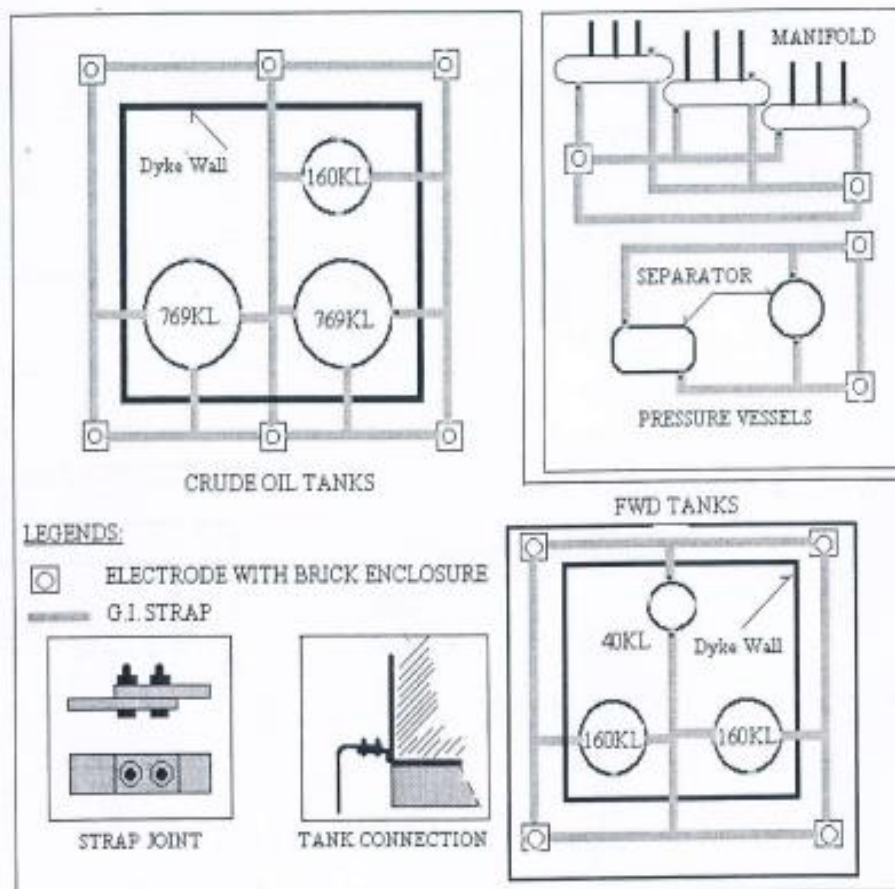
EARTH CONNECTIONS OF CRUDE OIL, FWD TANK AND PRESSURE VESSELS
