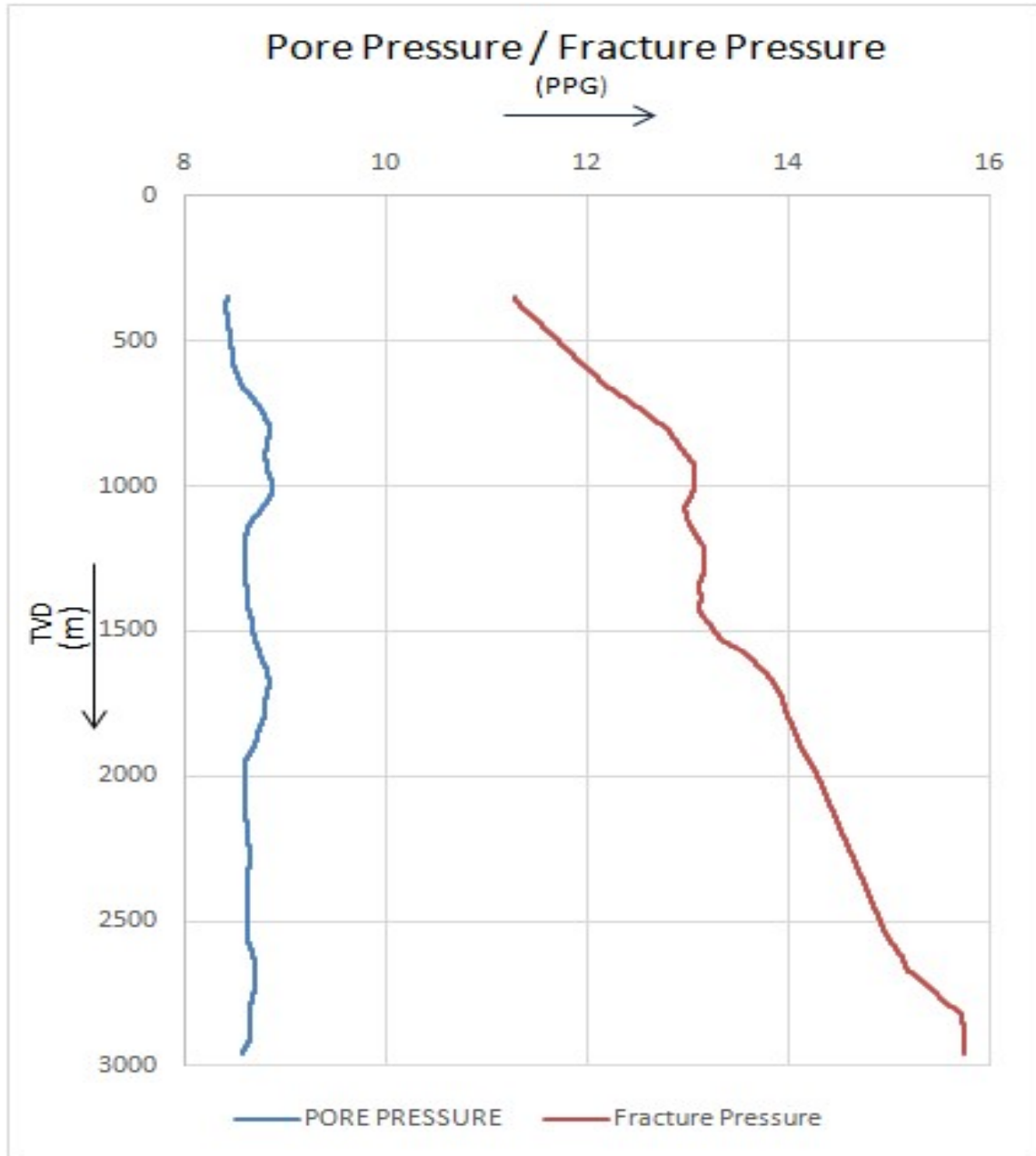
Figure (a): Average Pore pressure and fractured gradient in Mahanadi Onshore wells.
