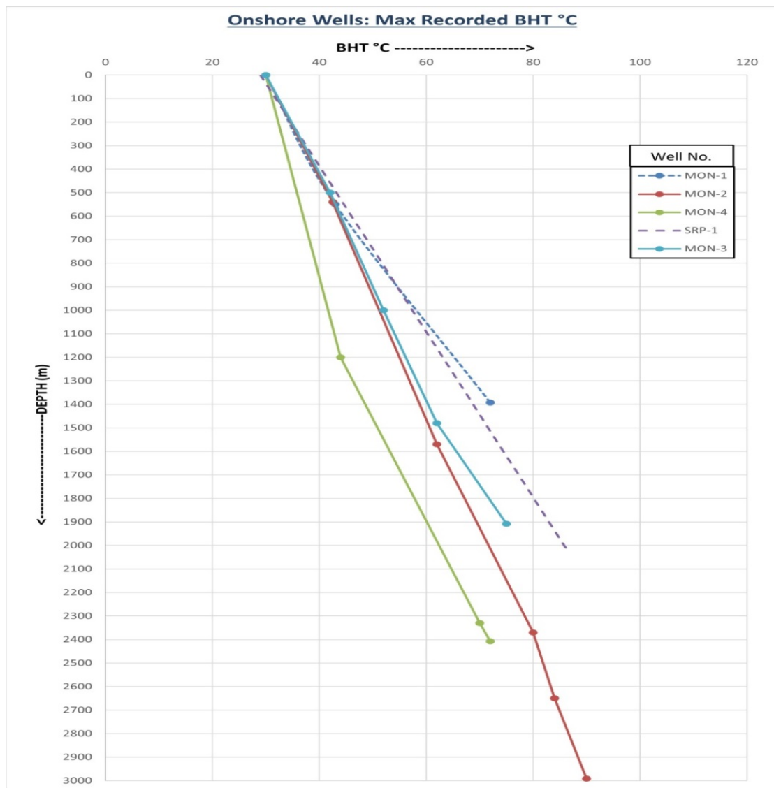
Figure-(b): Temperature profile in Mahanadi Onshore offset wells #Maximum BHT recorded in well MON#2 is 90°C at 2991.1m
