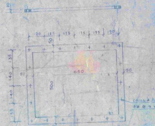
DETAIL OF MANHOLE DOOR FRAME
