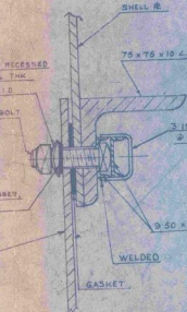
DETAIL AT-Y-Y
