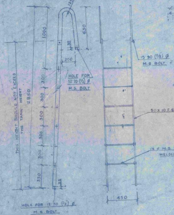
OUTER LADDER
