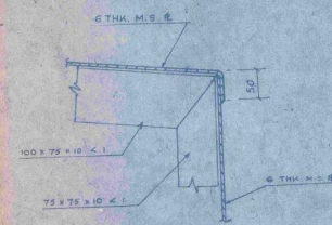
DETAIL OF MANHOLE COVER
