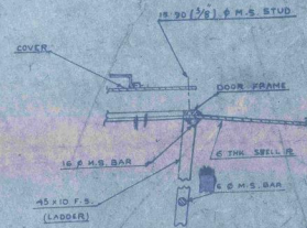
DETAIL AT-B
