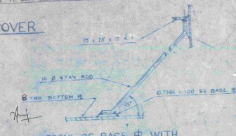
DETAIL OF BASE WITH STAY ROD
