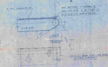
DETAIL AT Q
