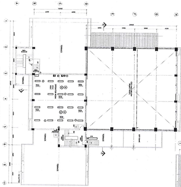
LIGHTING LAYOUT - FIRST FLOOR PLAN
