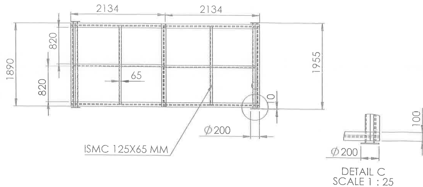
SKID -TOP VIEW
