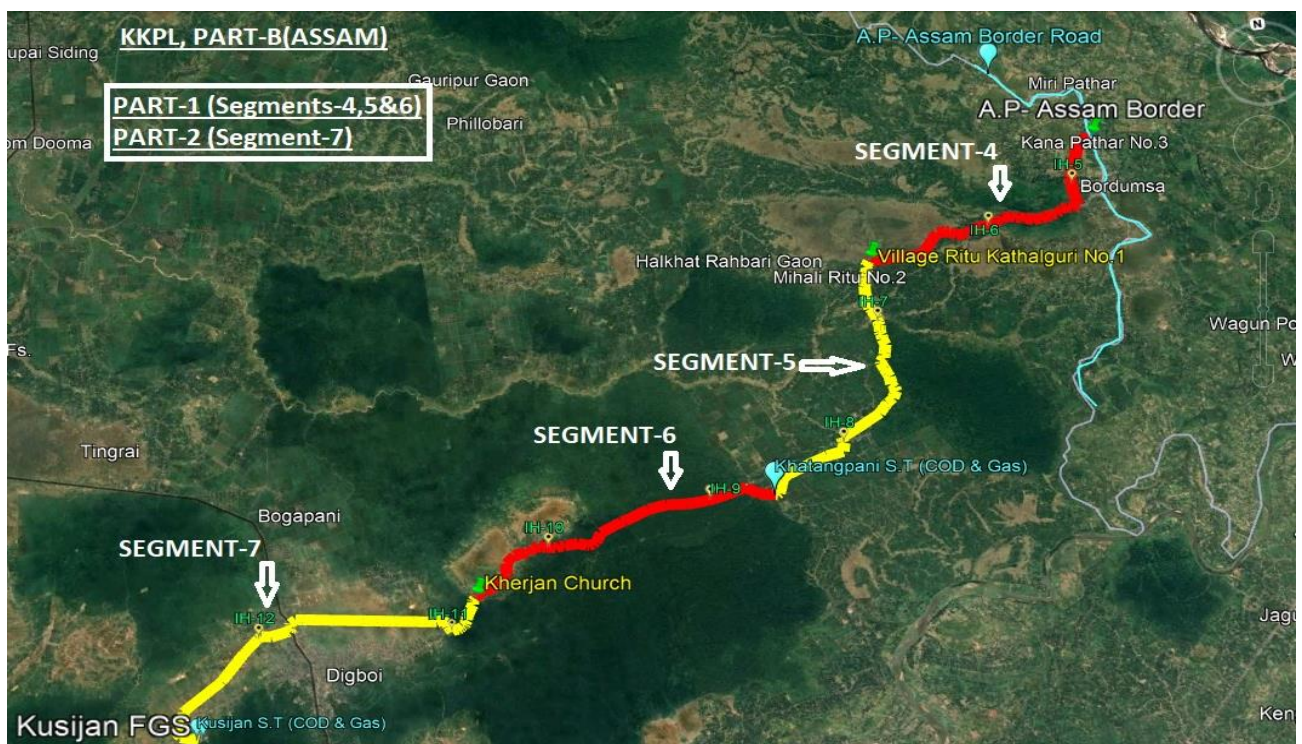
Fig: Showing KKPL, Part-B (Assam)'s, Part-1 (Segments 4,5&6) and Part-2 (segment-7) pipeline route.
