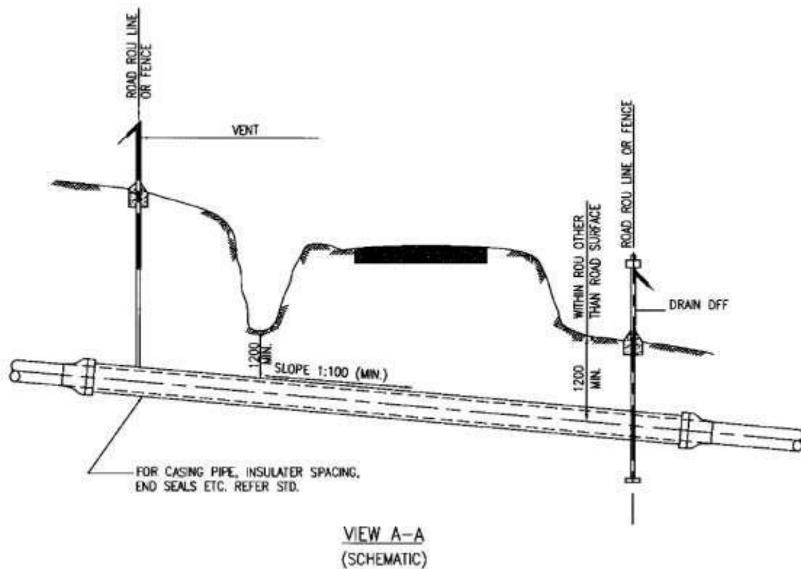
Fig.: Typical Pipeline Road Crossing (Cased) (dimension in mm)
