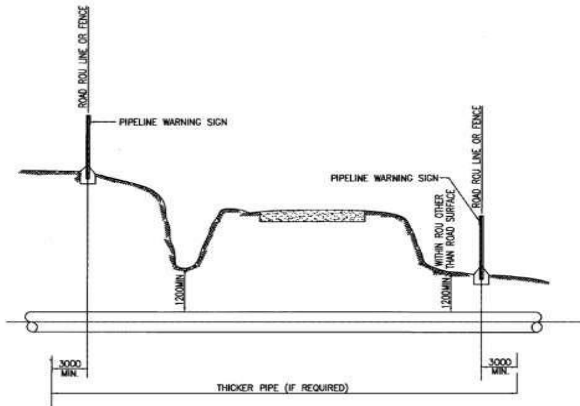
Fig.: Typical Pipeline Road Crossing (Uncased) (dimensions in mm)
