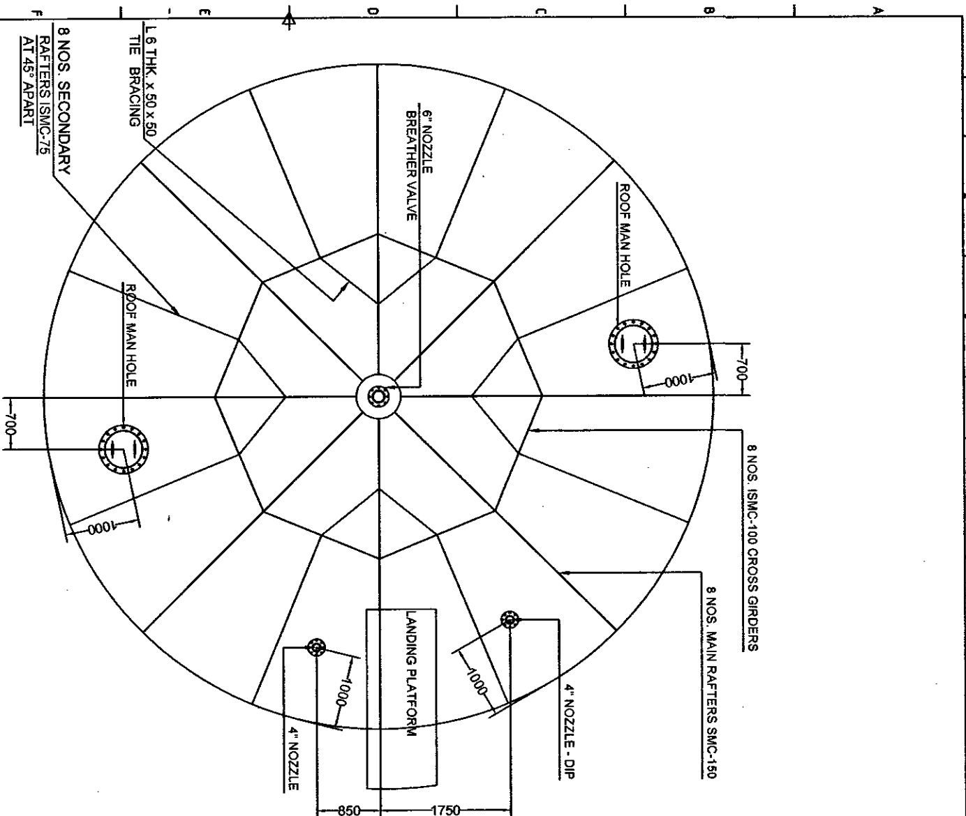
ROOF MAN HOLE & NOZZLE POSITION (TOP VIEW)
