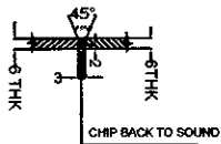
DET. OF SHELL HORIZONTAL WELD JOINTS (TYP)
