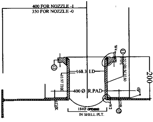
DETAIL OF NOZZLES - 0 & 1
