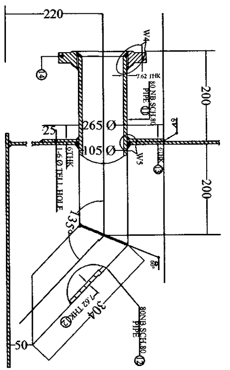
DETAIL OF SIPHON DRAIN
