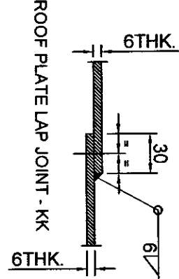
THREE PLTS. LAP JOINTS DETAIL DETAIL AT-X
