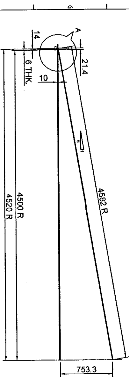
ROOF TO CURB ANGLE WELD DET.
