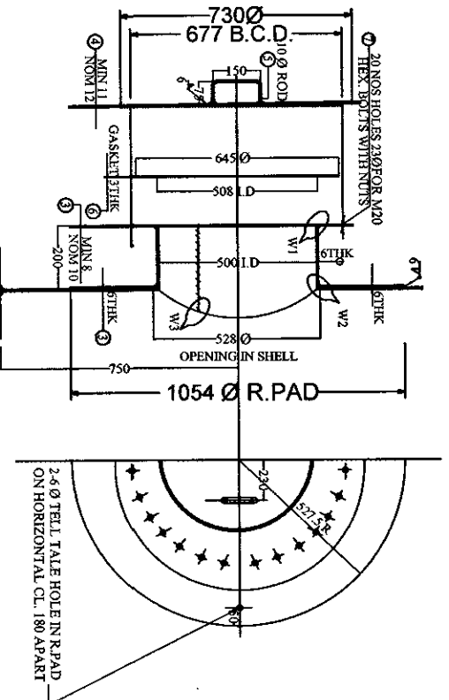
DETAIL OF MANHOLES - M1A/B HALF VIEW FROM -X
