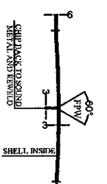
DET. OF VERTICAL WELD JOINTS
