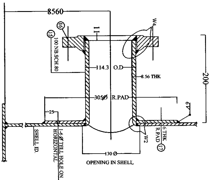
DETAIL OF NOZZLE-OF
