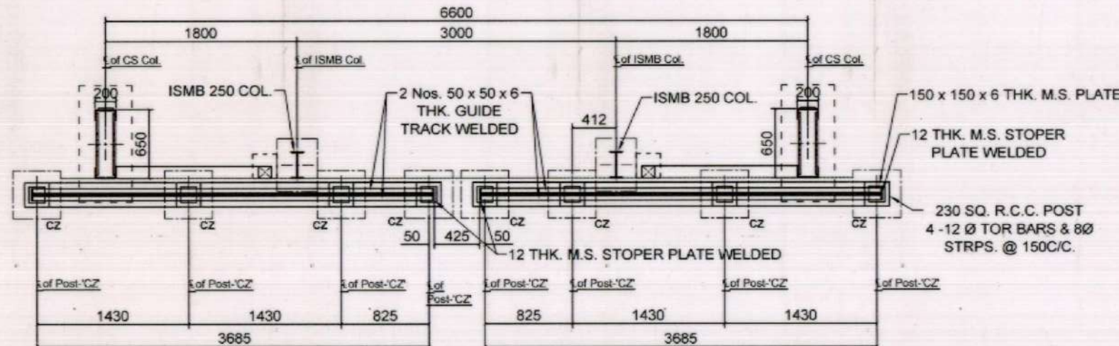
PLAN (SHOWING BOTTOM GUIDE ONLY)
