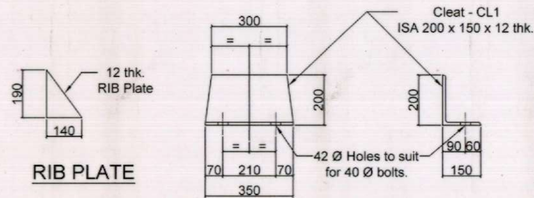
DETAILS OF CLEAT - CL1
