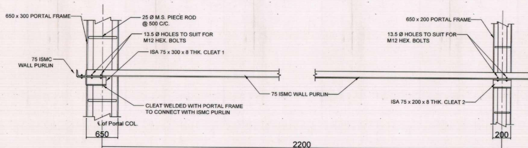
DETAILS OF WALL PURLIN - 'WP1'
