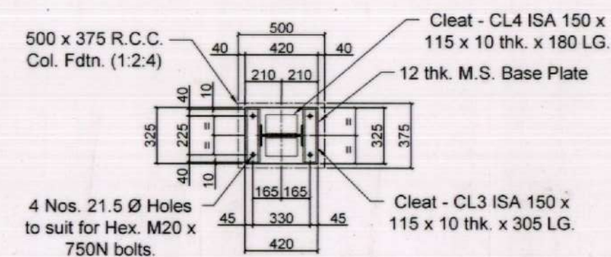
BASE PLAN (FOR ISMB COLUMN)
