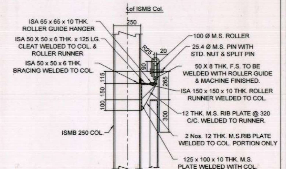
TYPICAL FIXING DETAIL OF TOP RUNNER
