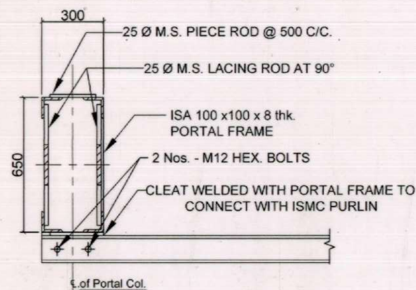
ENLRGD. CONNECTION DETAILS AT - 'X'
