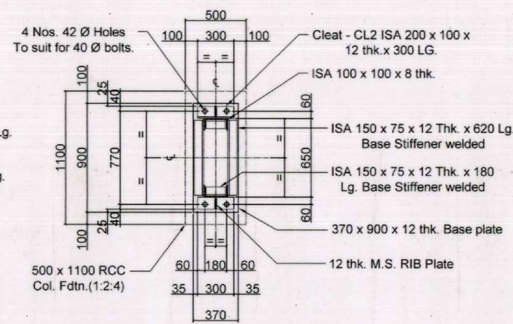
BASE PLAN (FOR CS COLUMN)
