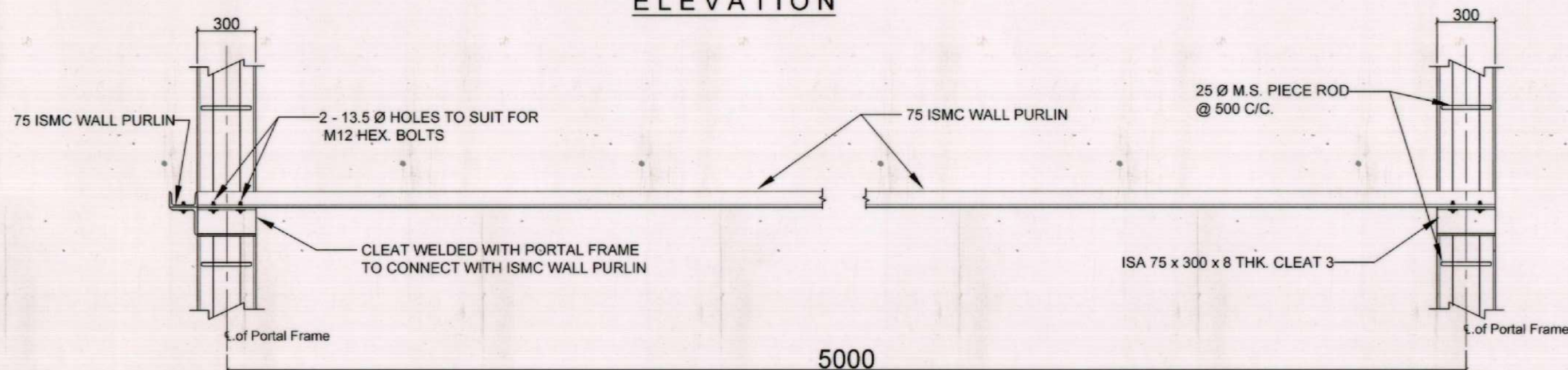
DETAILS OF WALL PURLIN - 'WP2'
