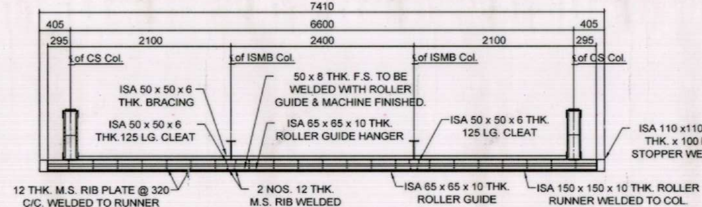
PLAN (SHOWING TOP GUIDE ONLY)
