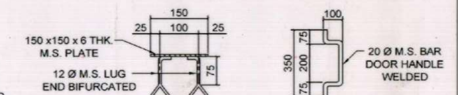
DETAIL OF M.S. PLATE WITH LUG
