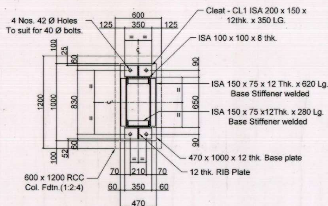
BASE PLAN (FOR PORTAL COLUMN)
