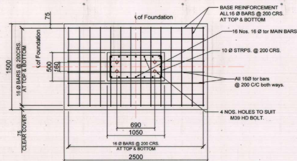
BASE PLAN
