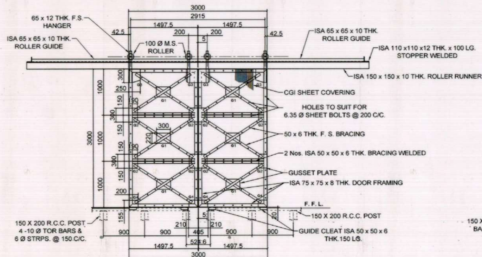
DETAIL OF SLIDING DOOR - SD1
