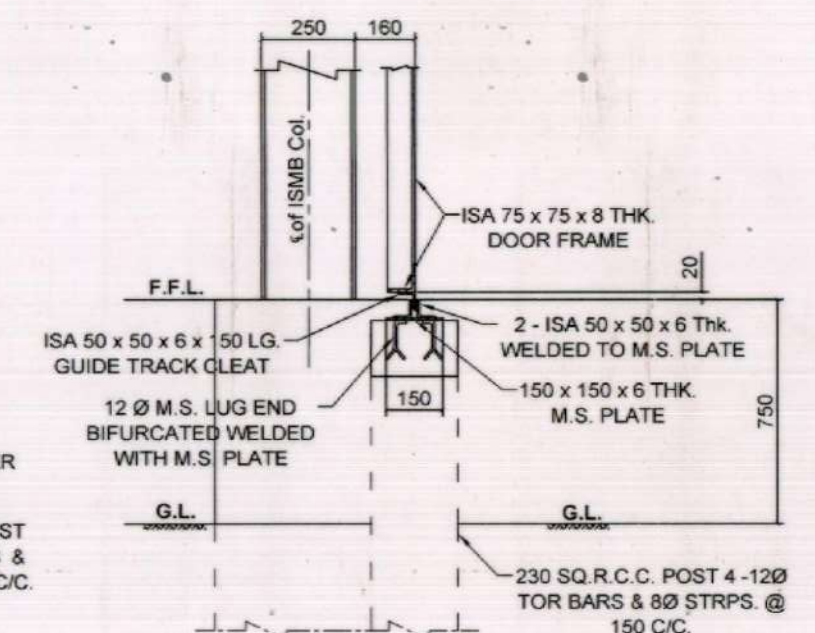
TYPICAL FIXING DETAIL OF BOTTOM RUNNER (FOR SLIDING DOORS - SD1 & SD2)
