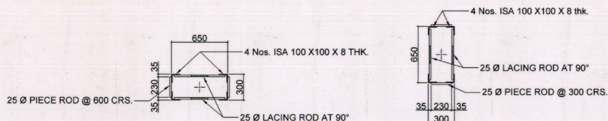
ENLGD. SEC. ON 'C-C'
