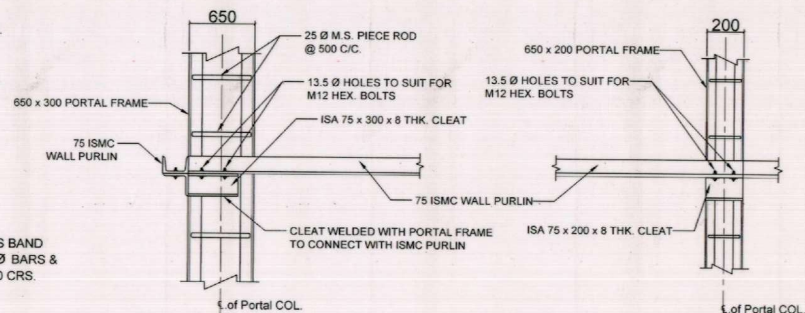
ENLRGD. DETAIL AT 'Y'
