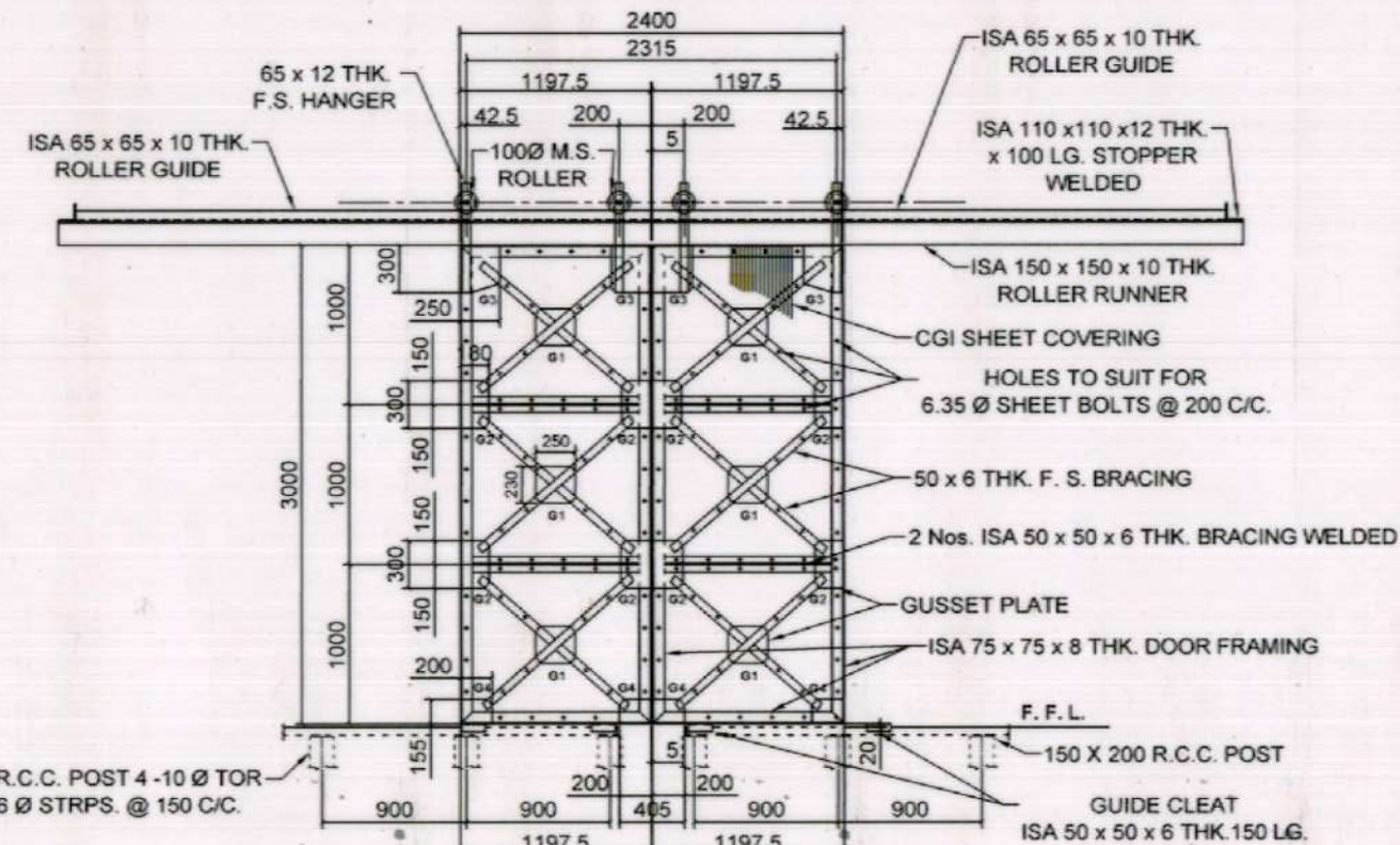
DETAIL OF SLIDING DOOR - SD2
