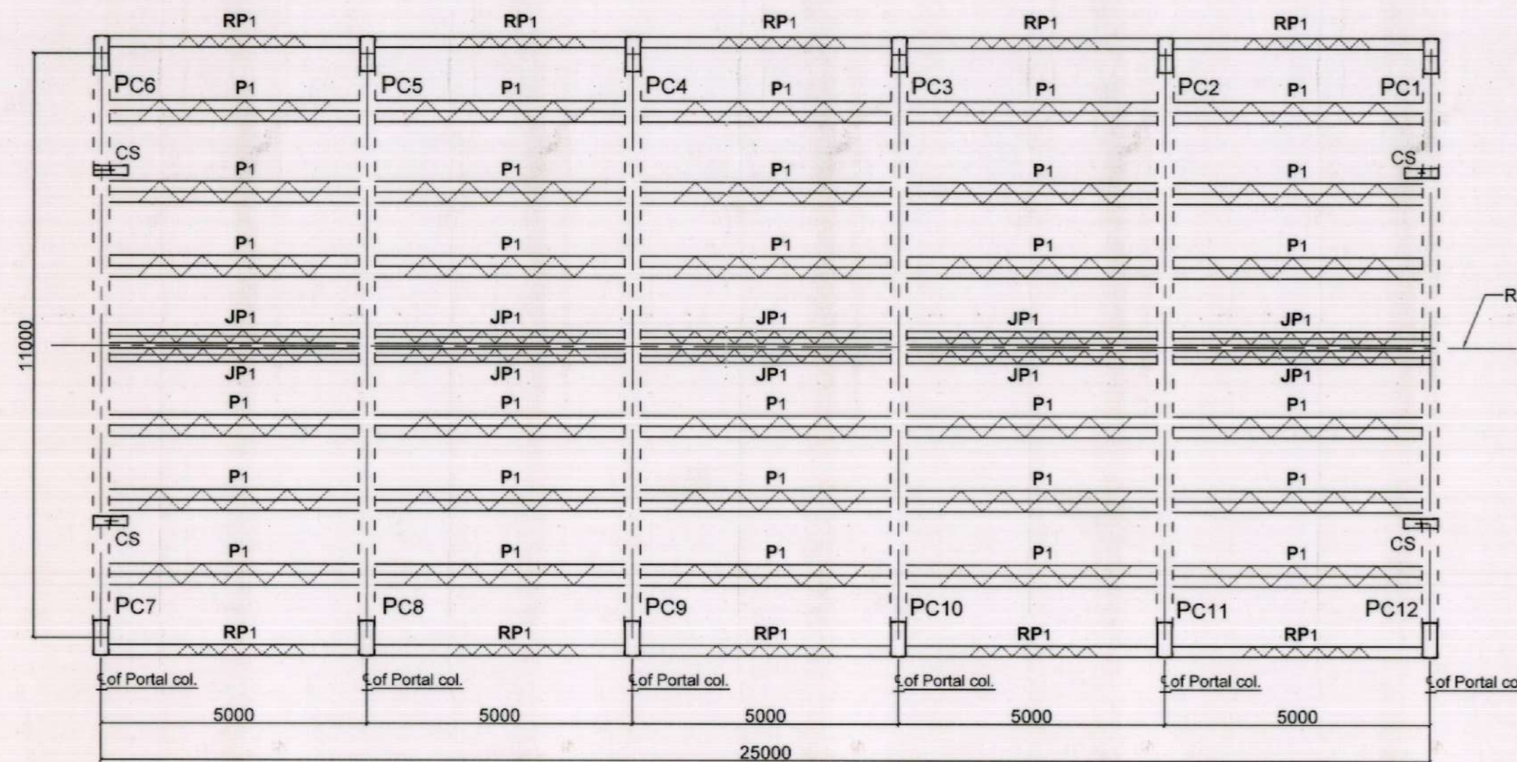
PLAN (SHOWING ROOF PURLIN ONLY)
