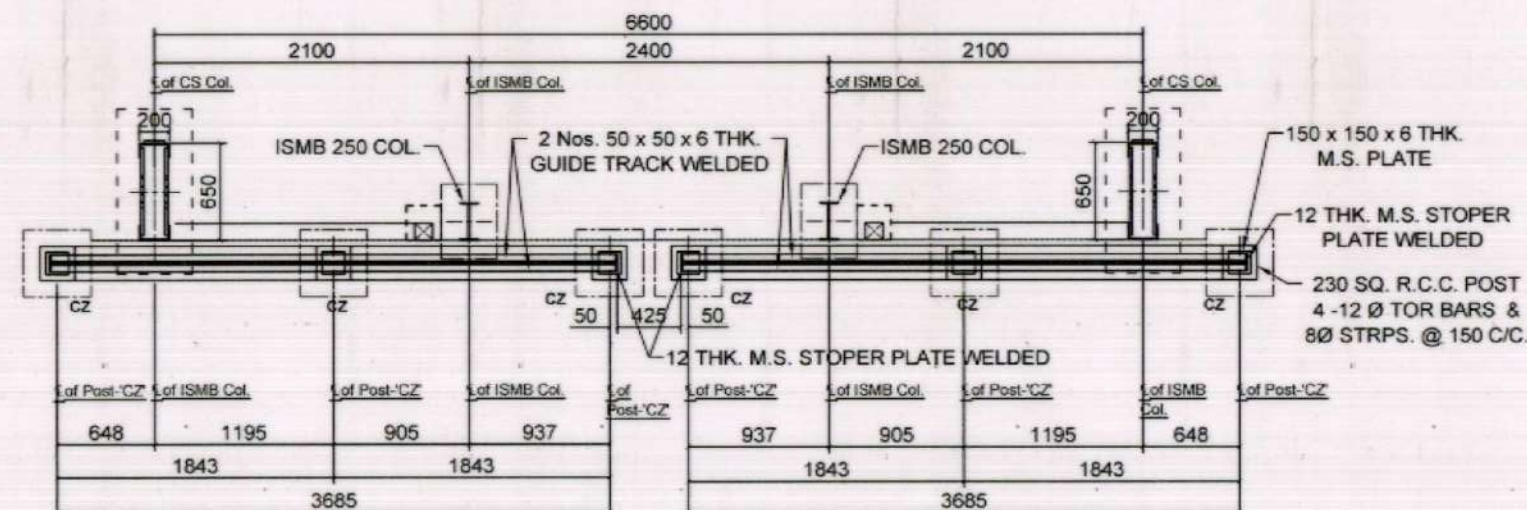
PLAN (SHOWING BOTTOM GUIDE ONLY)
