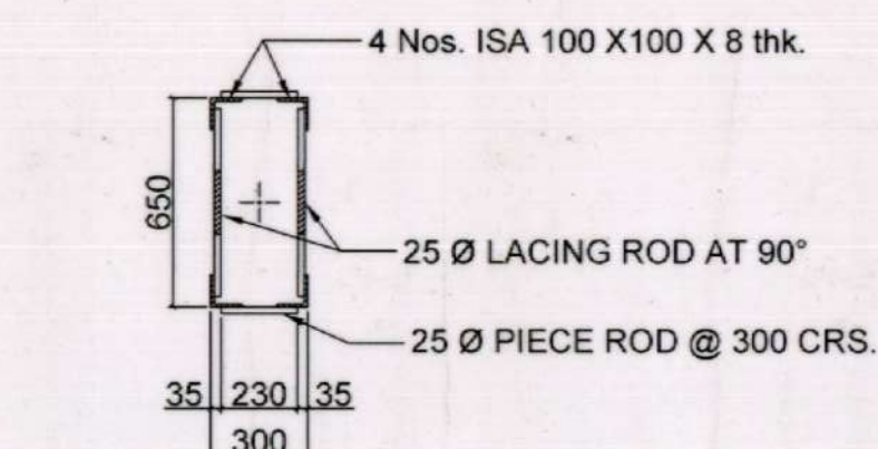
ENLGD. SEC. ON 'D-D'
