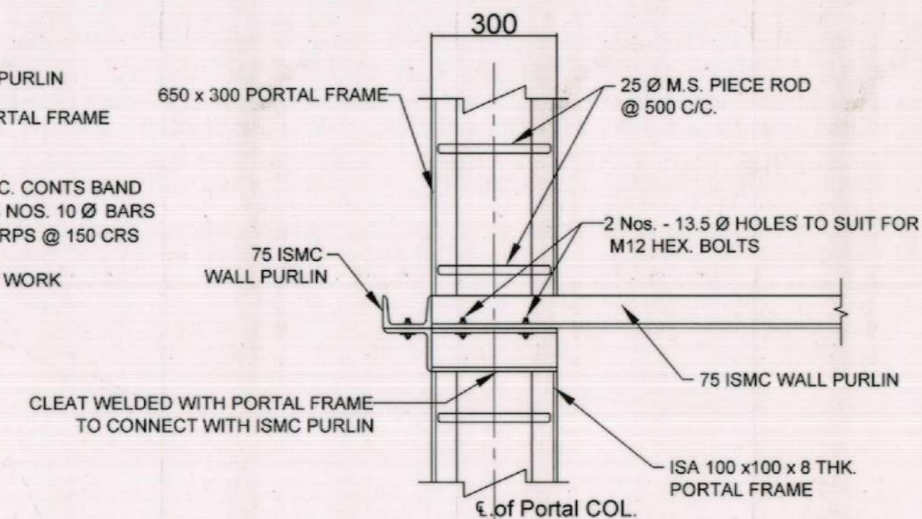
ENLRGD. DETAIL AT 'X'
