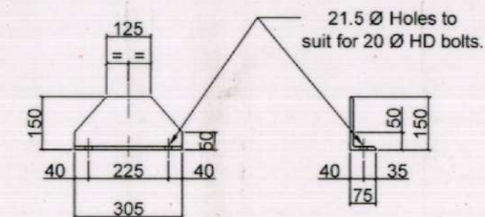
DETAILS OF CLEAT - CL3
