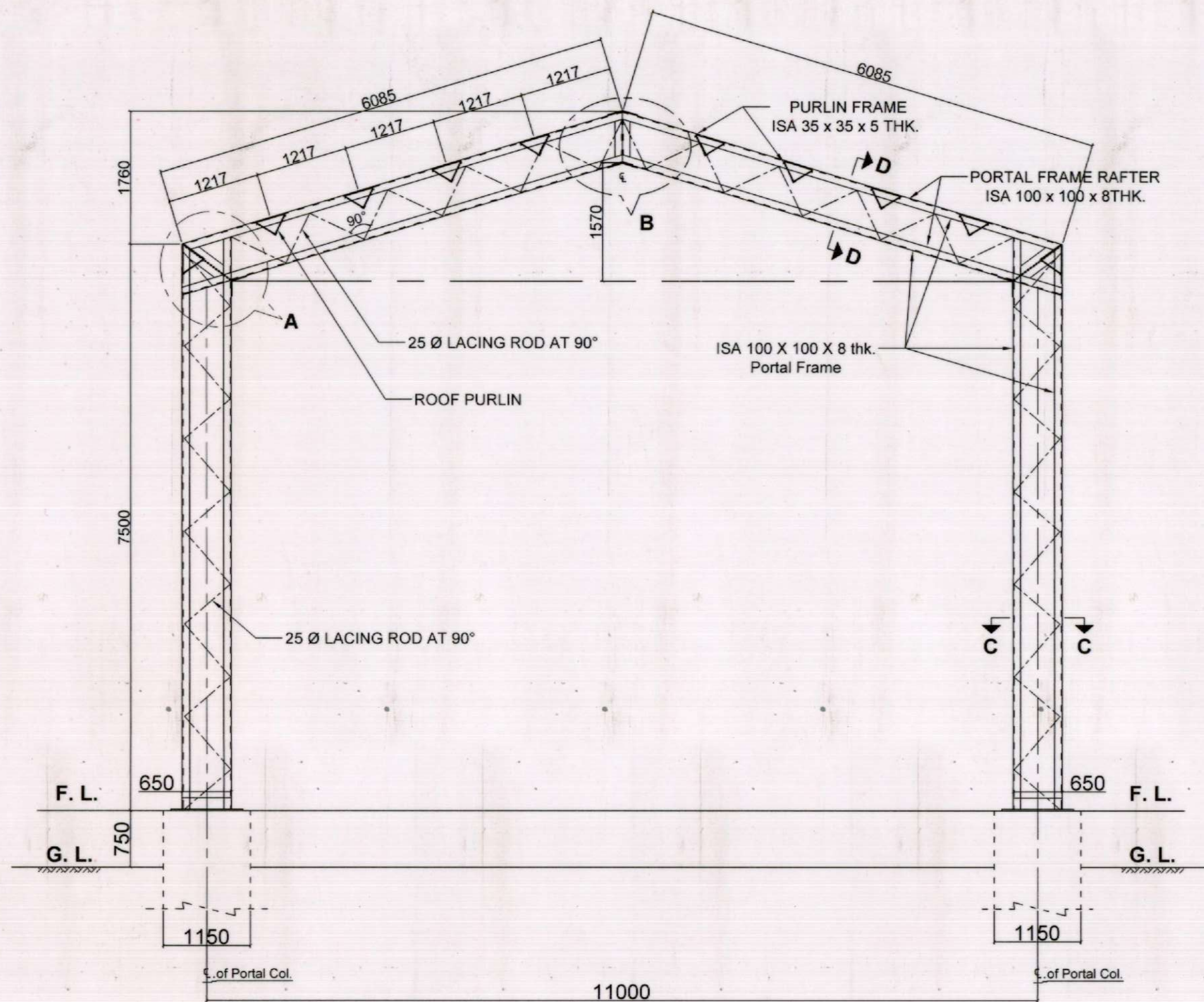
DETAILS OF PORTAL FRAME
