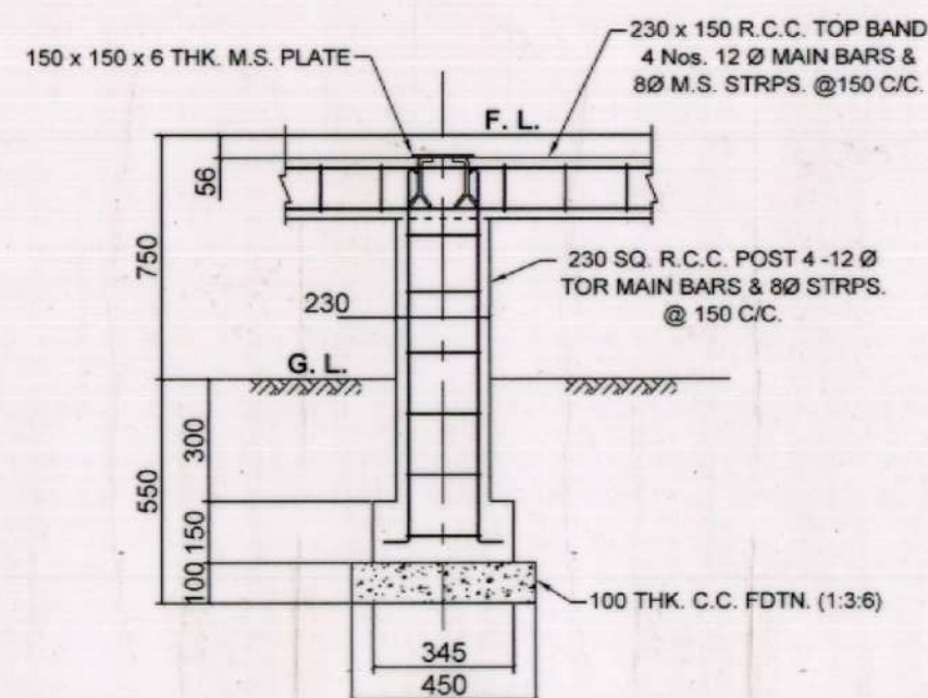
DETAIL OF 230 SQ. R.C.C. POST - 'CZ'
