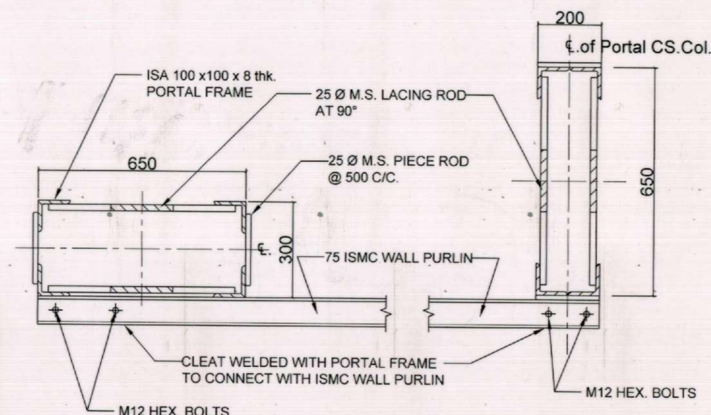
ENLRGD. CONNECTION DETAILS AT - 'Y' - 'Z'
