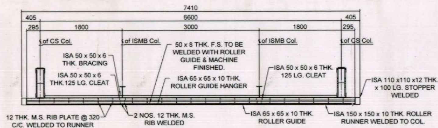
PLAN (SHOWING TOP GUIDE ONLY)
