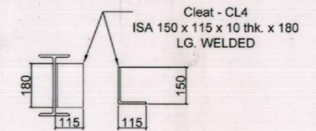
DETAILS OF CLEAT - CL4
