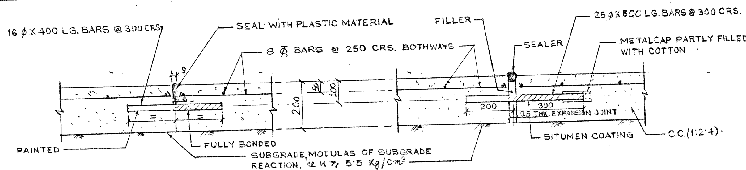
SEC. 2-2 (EXPANSION JOINT)
