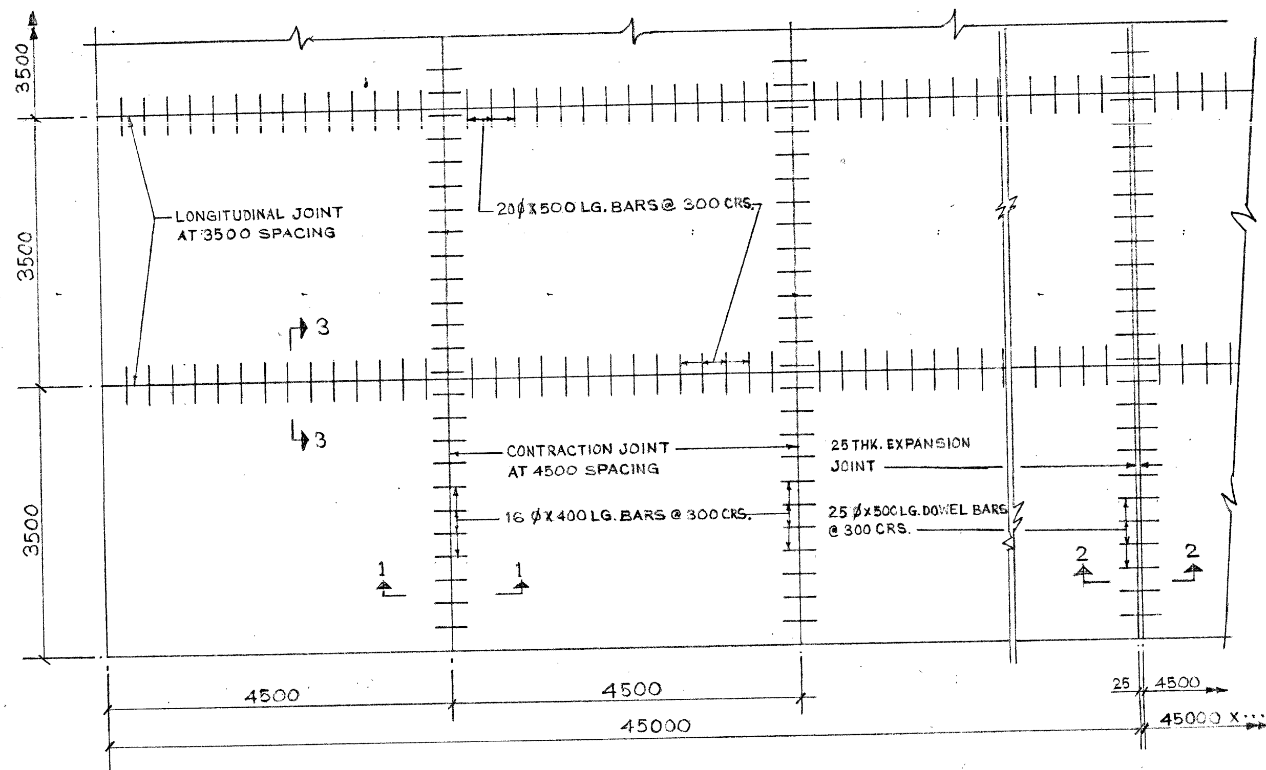
PLAN
