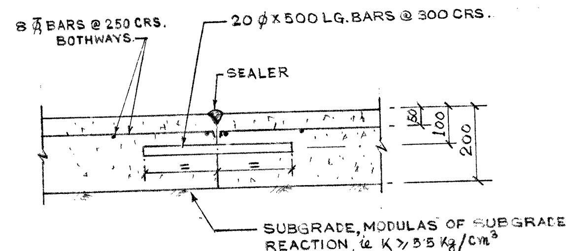
SEC. 3-3 (LONGITUDINAL JOINT)
