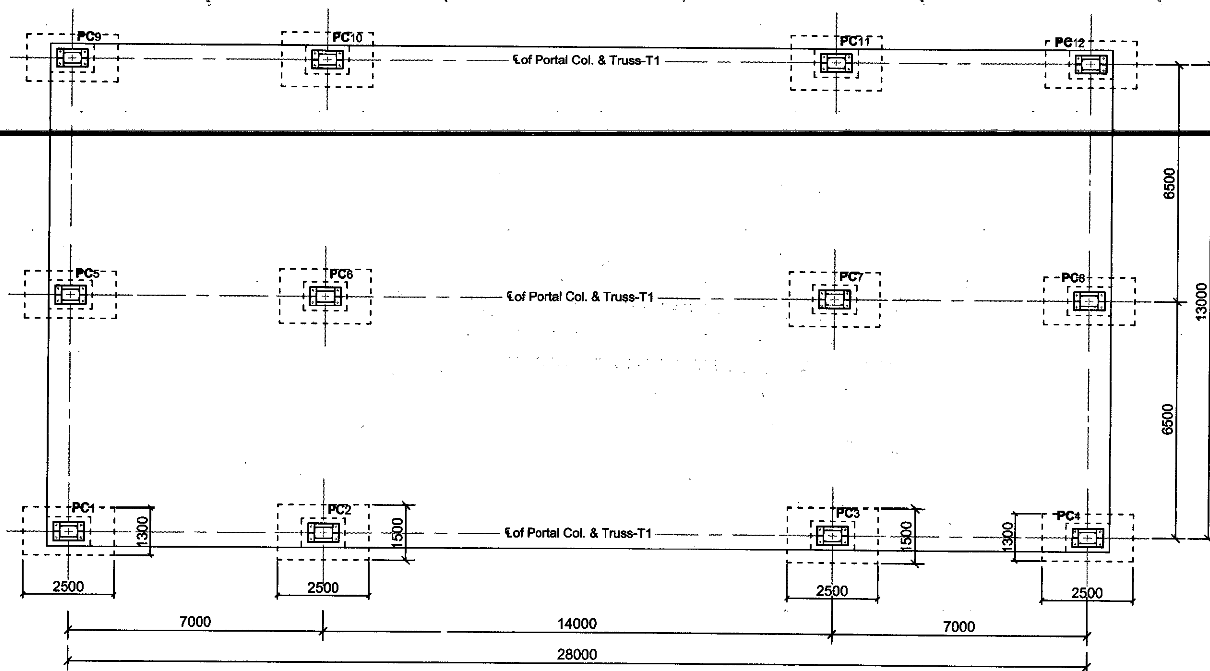
PLAN
