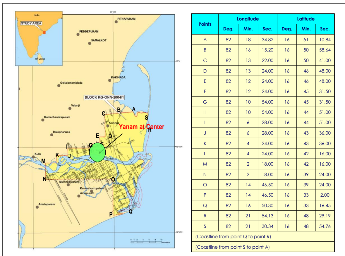
Figure-1a: The location of the Block KG-ONN-2004/1 in KG basin
