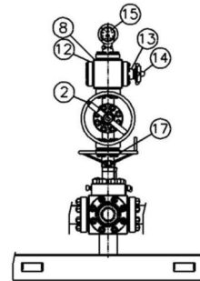
DETAIL 'A-A'
