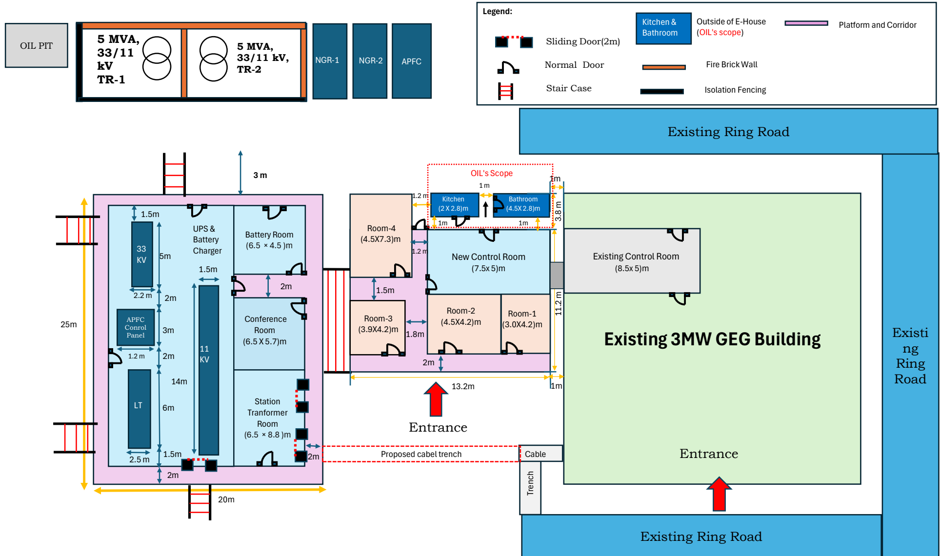
A21.1(A): Layout Diagram- E-House(OIL, Moran)
