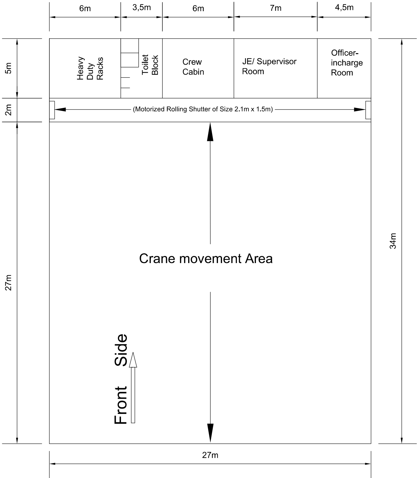
PEB Shed Rig Building Section (representative diagram)
